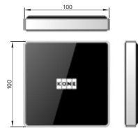
Surface mount landing call station (LCS) with- out key switch
