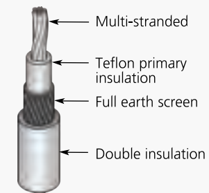
Wire Cross-Section
